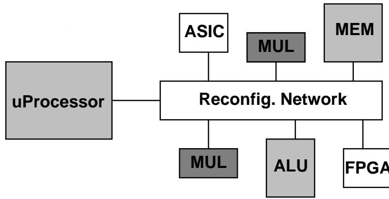
Figure 6: Architectural template for a single-chip Pleiades device [103].
