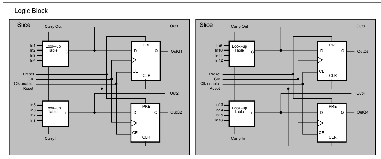
Figure 2: Simplified Xilinx Virtex logic block [111]. Each logic block consists of two 2-LUT slices.
