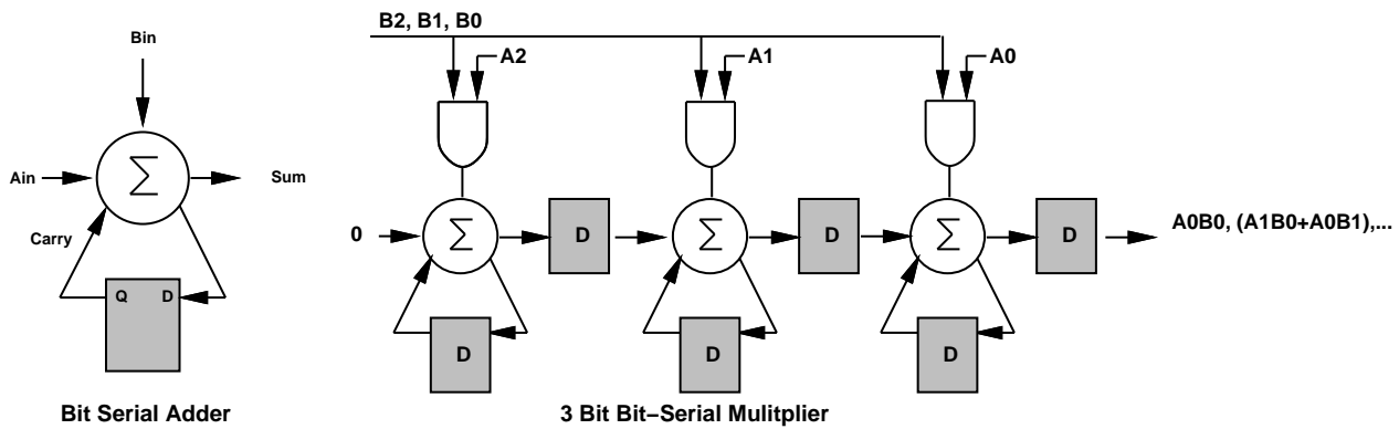
Figure 4: Bit-serial adder and multiplier [74].
