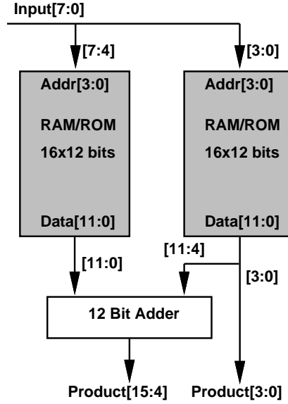
Figure 5: Distributed arithmetic multiplier [74].
