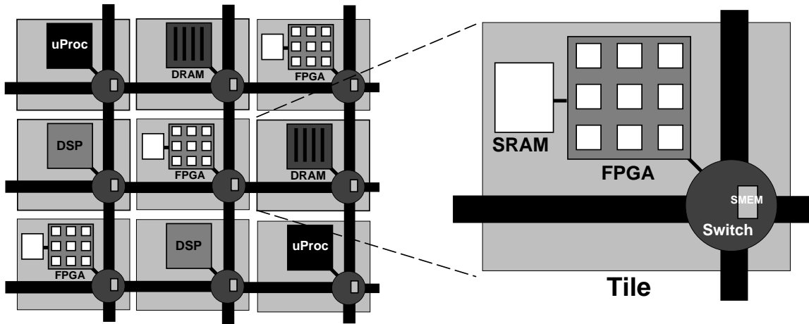
Figure 7: Distributed single-chip DSP interconnection network [93].
